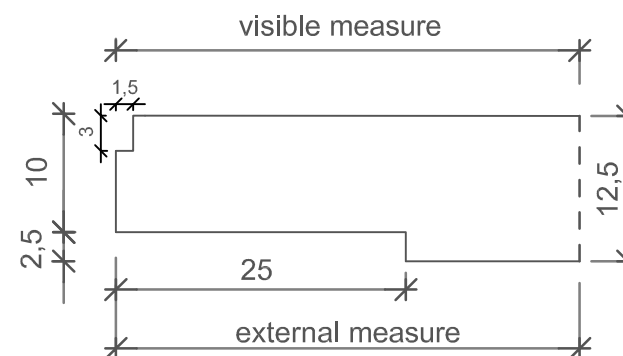
Detail B
