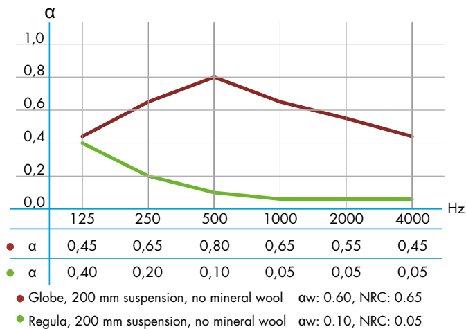
Edge B (bevelled edge) Visible joints For Globe
