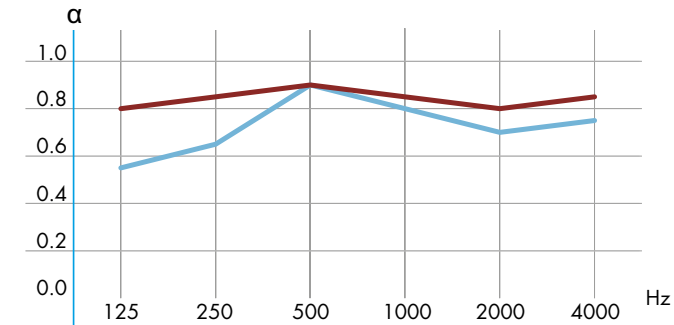
Edge B (Bevelled edge) Visible joints
