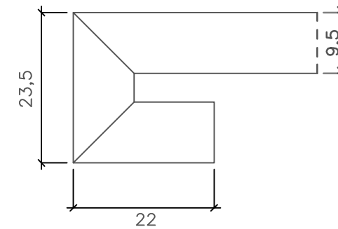
Detail C
