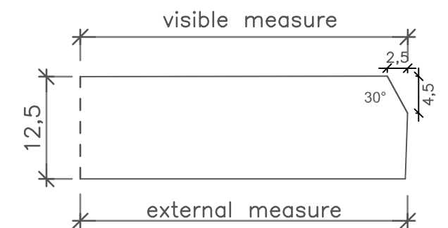
Detail C
